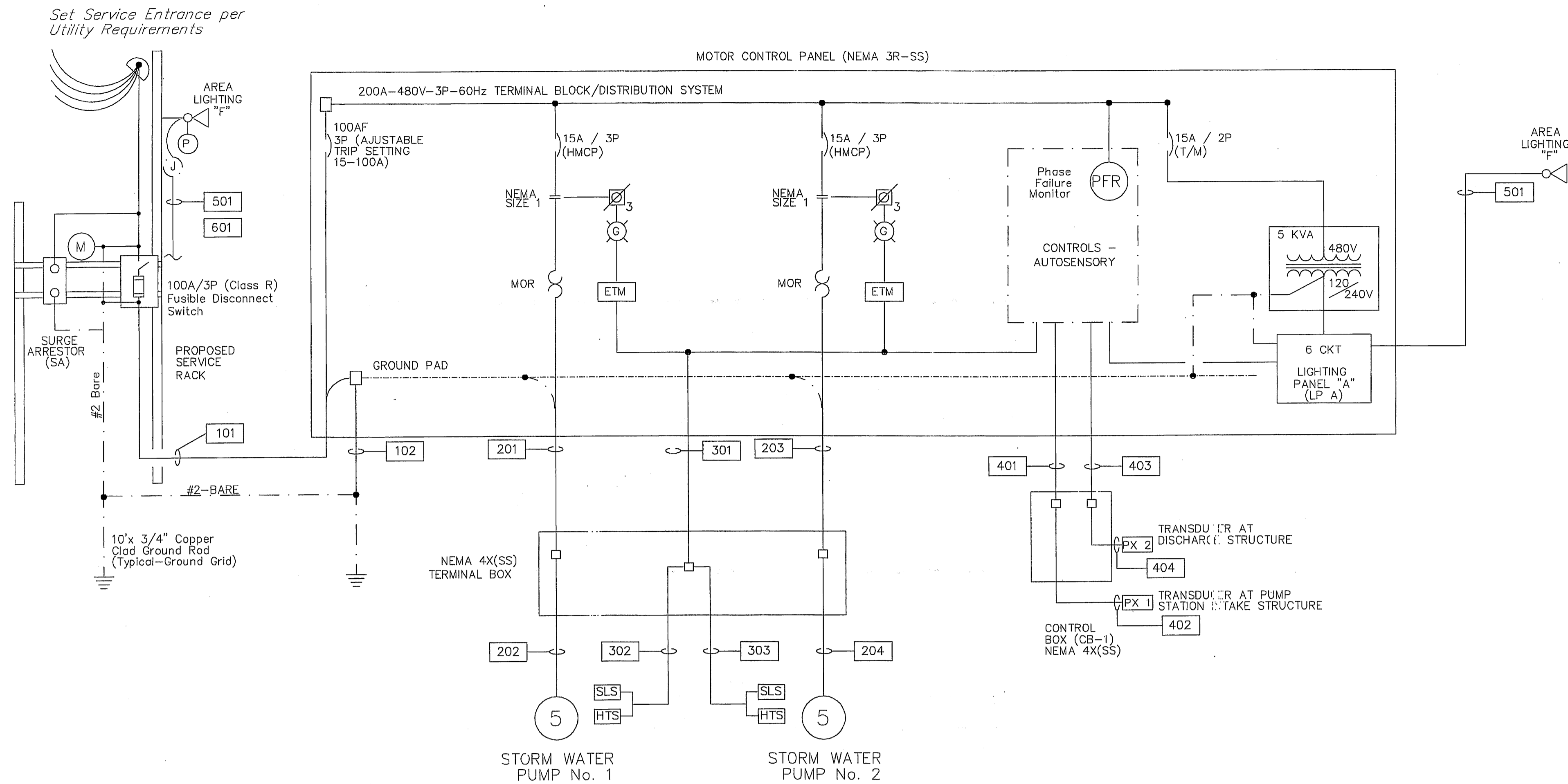
MOTOR CONTROL CENTER ONE-LINE DIAGRAM
