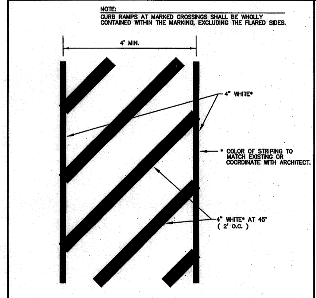
CROSSWALK DETAIL No. 103 SIDE WALK CONTROL & EXP. JOINT No. 167
