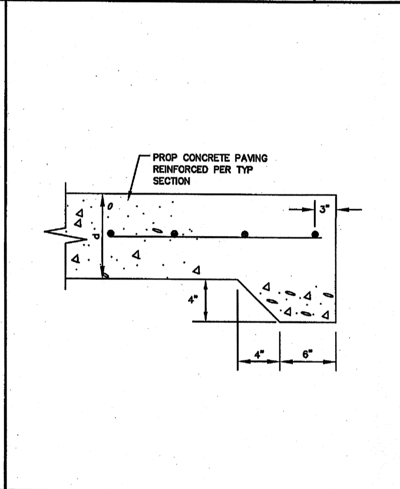
CONCRETE PAVING CRACK CONTROL JOINT No. 132 SANITARY SEWER BLOCKOUT DETAIL No. 200
