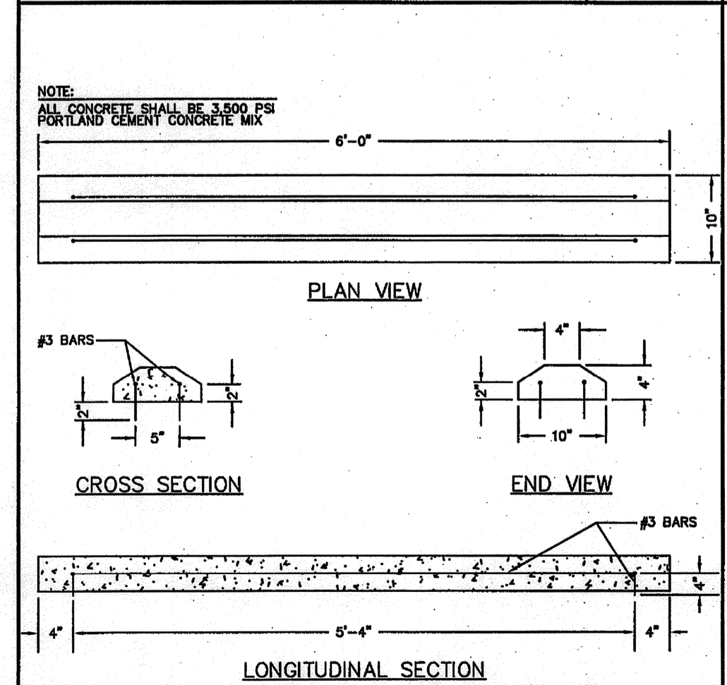
WHEEL STOP DETAIL No. 144 GRATE INLET JOINT & CURB DETAIL No. 143
