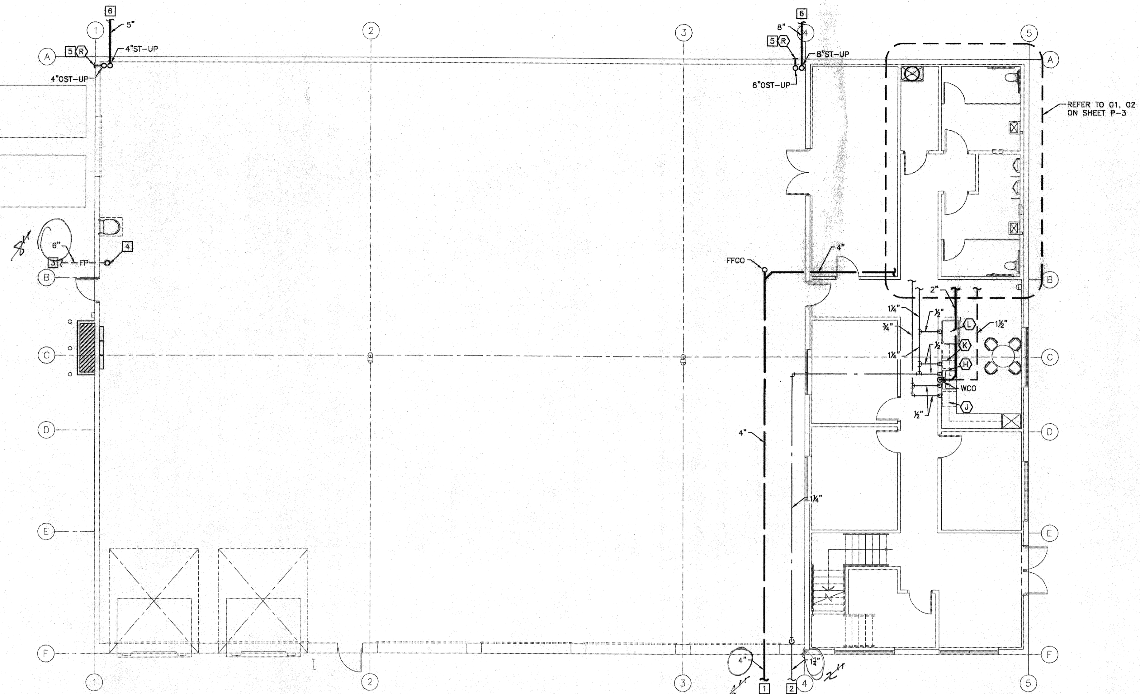
01 FIRST FLOOR PLUMBING PLAN 1/8" = 1'-0" NORTH TRUE
